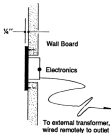
Flush Mount Cross-Section
